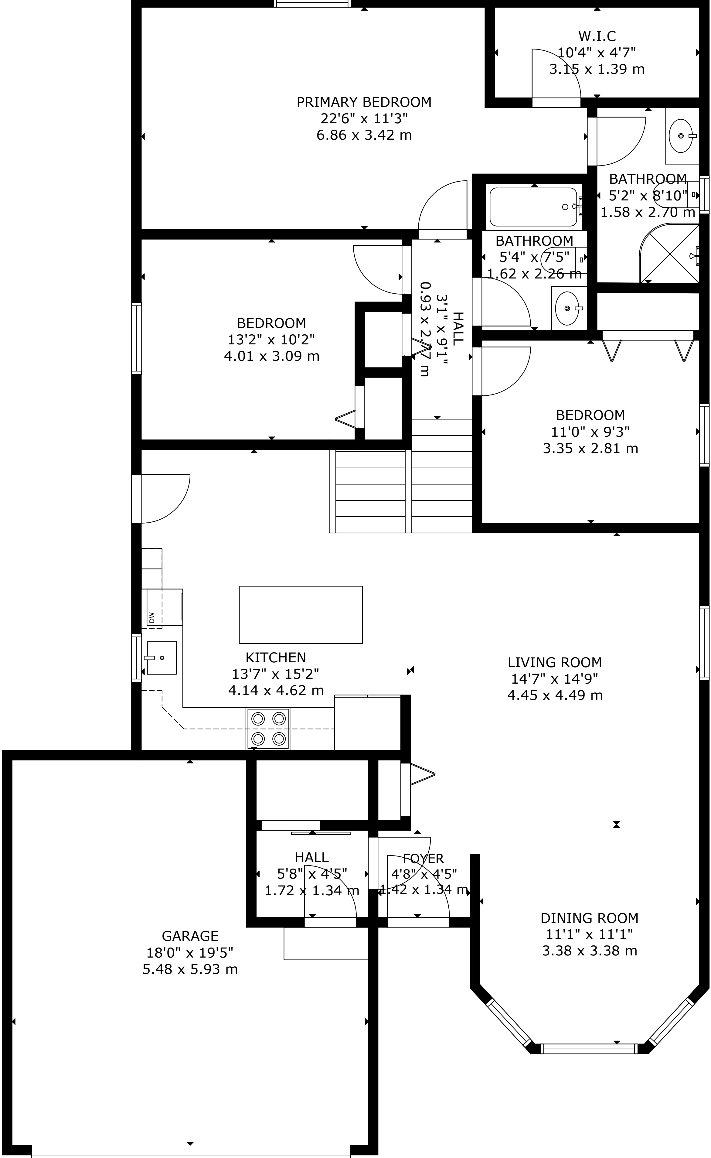
FIRST FLOOR
